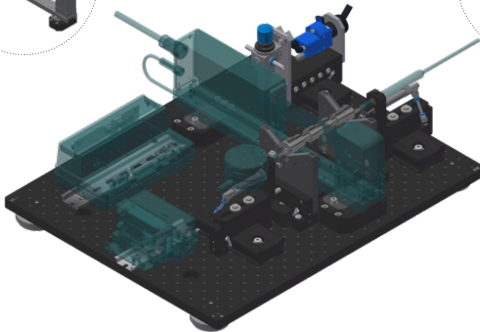
K551377 Measuring slide digimatic indicator*
